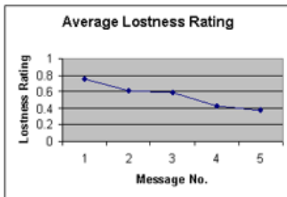
Fig. 10. Average lostness rating for five sequence messages during experiments
