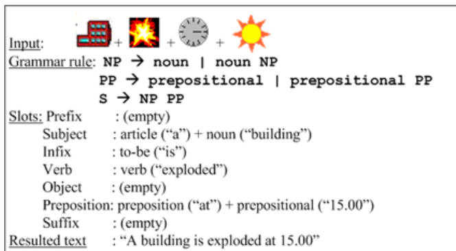
Fig. 3. An example of an icon string input conversion
