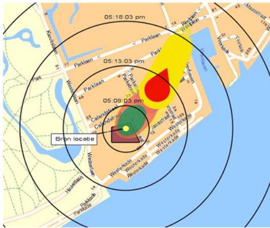
Fig. 8. An example of gas dispersion scenario shown by the simulator's interface
