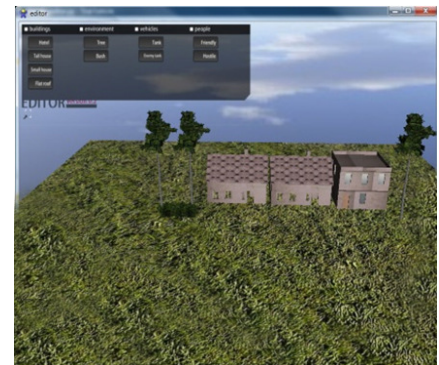
Figure 6-2: Example scene
