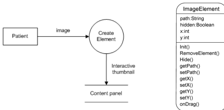
an image Figure 5-12: ImageElement class
