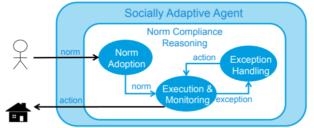
Figure 1: Socially Adaptive Agent Architecture
