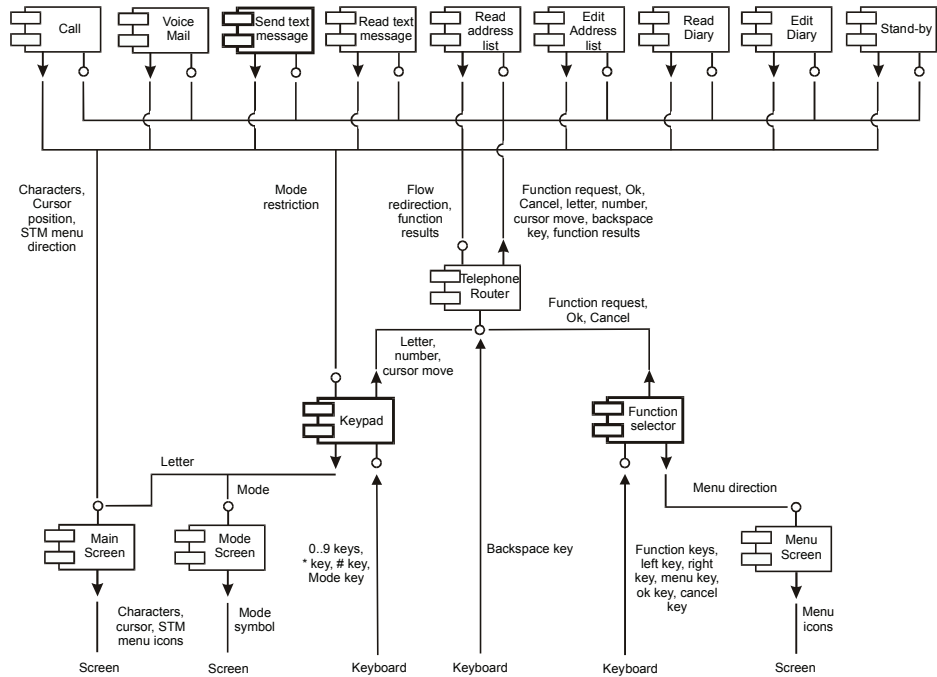
Fig. 4. The architecture of the Mobile telephones (bold interaction components were manipulated in the experiment).
